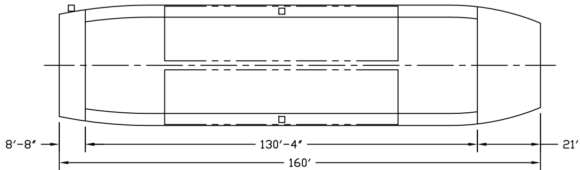
BARGE R22 ARRANGEMENT 1/32" = 1'-0"
