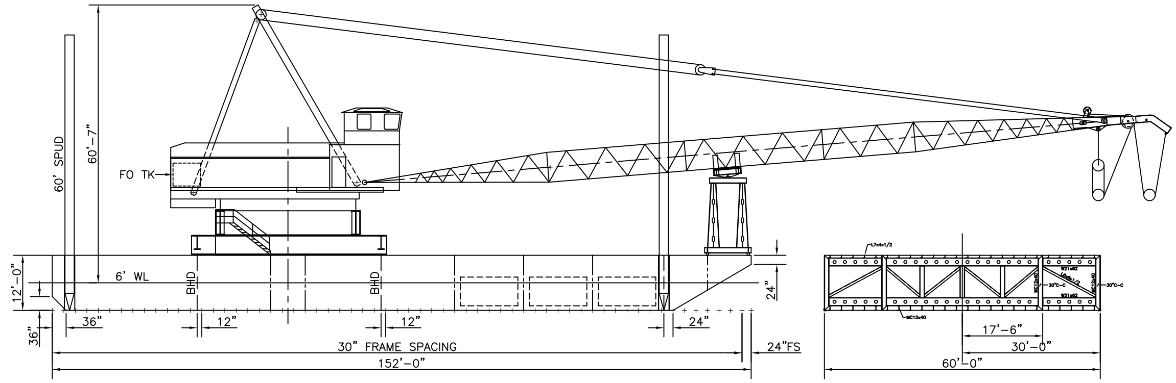
ELEVATION 1-5A PROFILE BARGE w/CRANE
