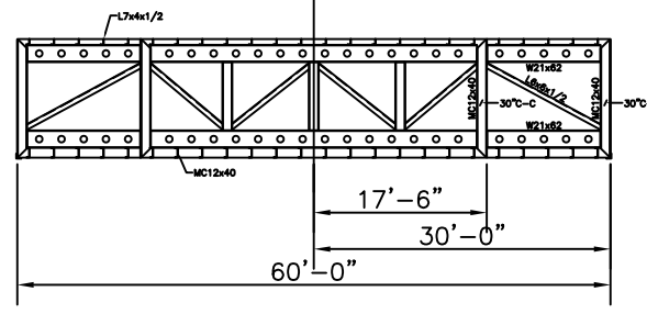
SECTION 1-3A TYPICAL FRAME
