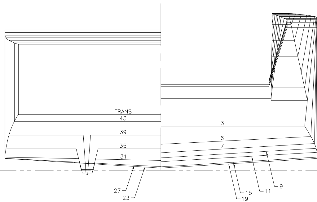
BODY LINES 1/4"=1'-0"
