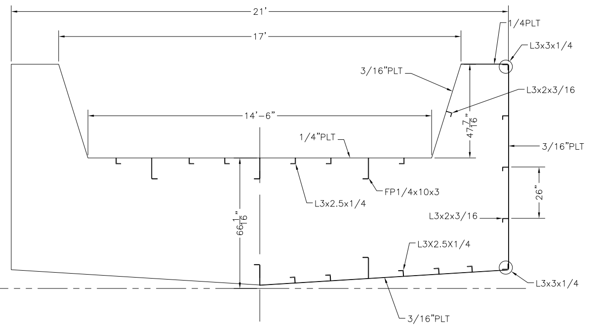
STRUCTURAL SECTION FRAME 23 1/4"=1'-0"
